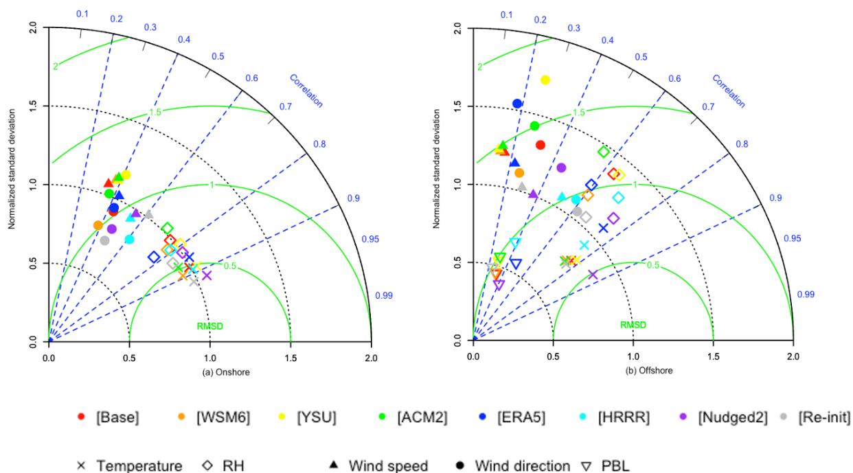
Figure 5. Assessments of meteorological variables simulated by the WRF model configurations against (a) CAMS hourly measurements and (b) boat 1-minute measurements for all sites during high ozone days. Green, black, and blue lines indicate contours of the normalized centered root-mean-square differences (RMSD), the normalized standard deviations, and the correlation coefficients, respectively. The reference point representing observed state is plotted at 1 along x axis, and the distances to reference point show model performance.
