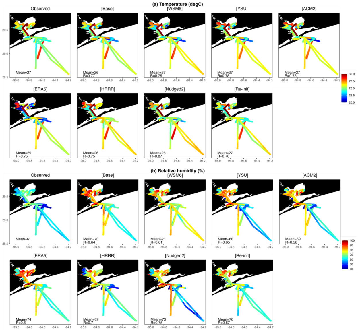
Figure 3. Spatial distribution of boat-observed and modeled meteorology during ozone episodes.
