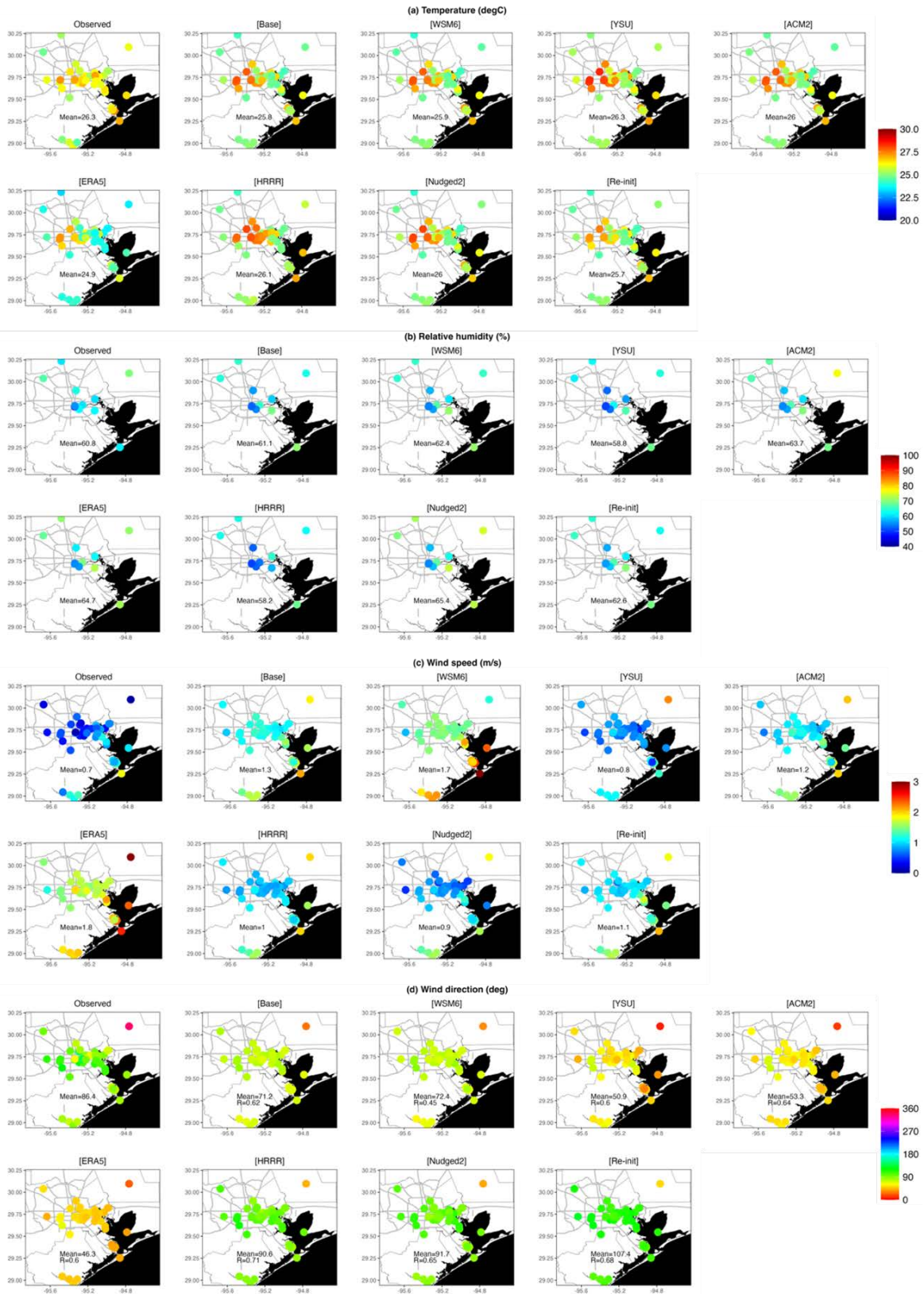
Figure 1. Spatial distribution of CAMS-observed and modeled mean meteorology during ozone episodes.
